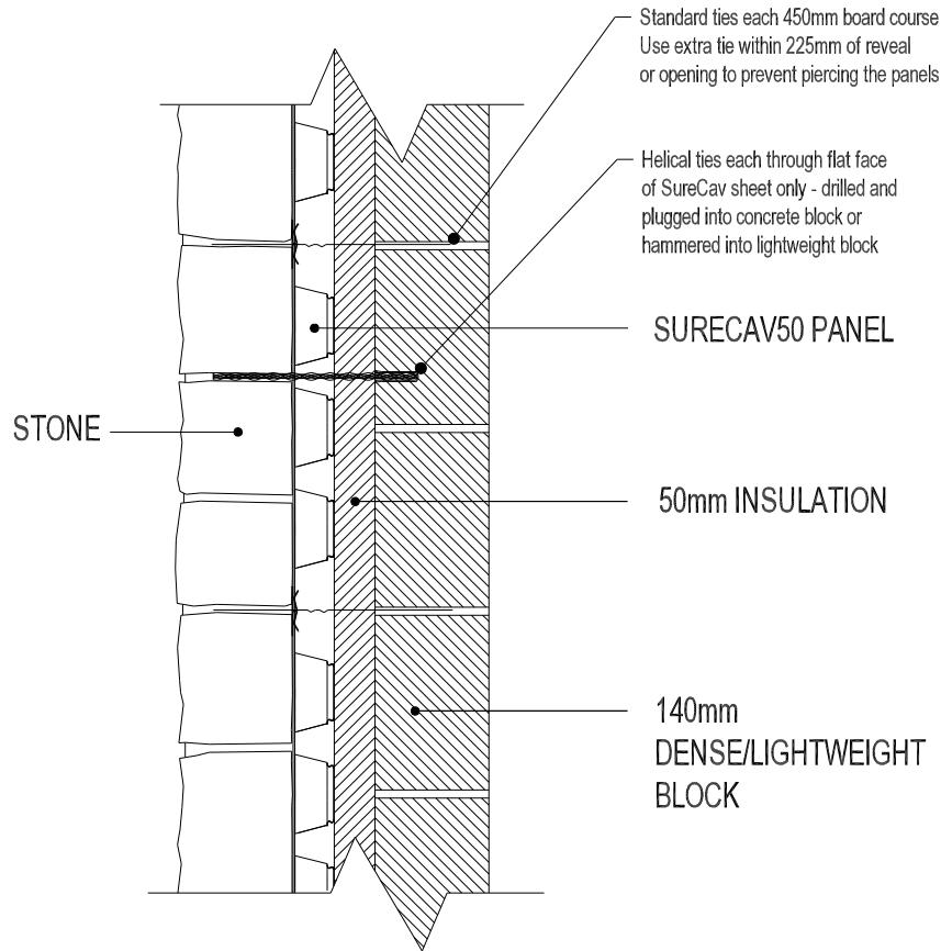
SURECAV50 WALL-TIE OPTION WITH DENSE OR LIGHTWEIGHT BLOCKS
