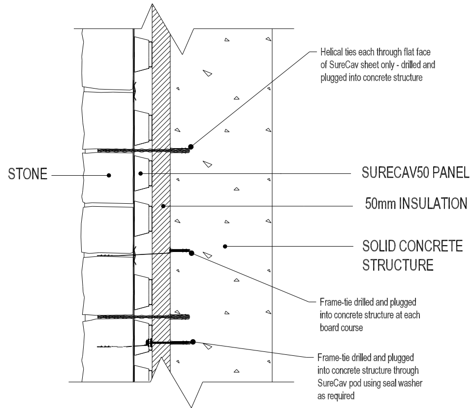
SURECAV50 WALL-TIE OPTION WITH SOLID CONCRETE STRUCTURE
